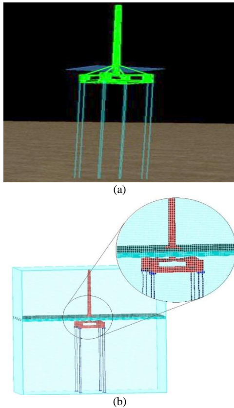
Figure 4. Mesh details of TLP (a) BEM (b) FVM.
