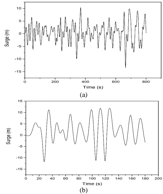
Figure 11. Time history of platform surge motion in 100-year irregular wave using (a) BEM (b) FVM.
