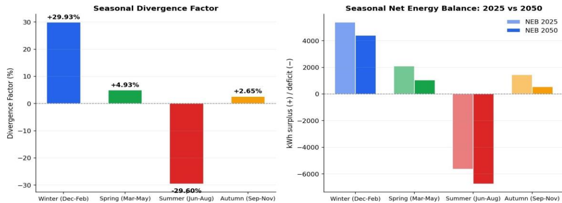
Figure 6. Seasonal net energy impact: 2025 vs. 2050. The winter surplus masks the summer deficit when only annual values are reported.
