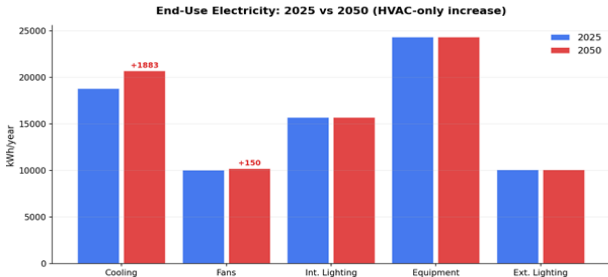
Figure 3. Projected end-use electricity demand: 2025 vs. 2050. Only HVAC-related end-uses change between epochs.
