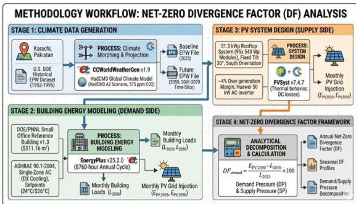
Figure 1. The integrated four-step simulation pipeline used to calculate the Net-Zero DF.
