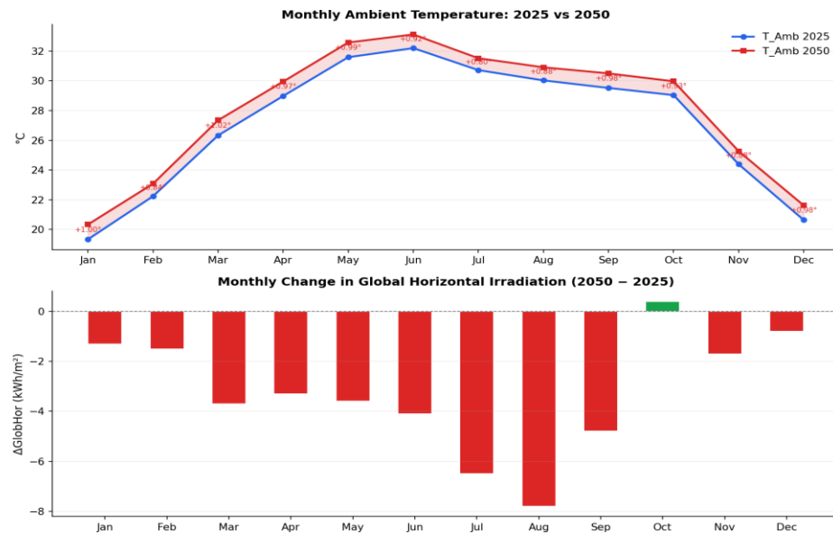
Figure 2. Comparative analysis of climate parameters (2025–2050) derived from CCWorld-WeatherGen HadCM3 A2 morphing.
