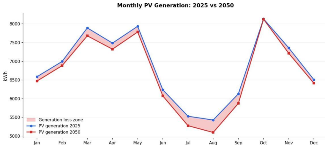
Figure 4. Impact of climate change on monthly PV generation (2025–2050).
